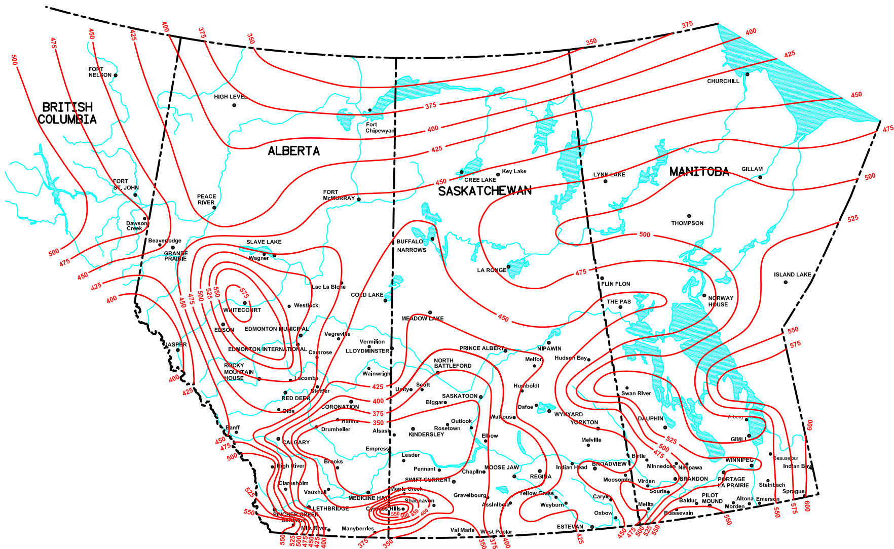
MEAN ANNUAL PRECIPITATION (mm) IN THE CANADIAN PRAIRIES FOR THE STANDARD PERIOD 1971-2000
