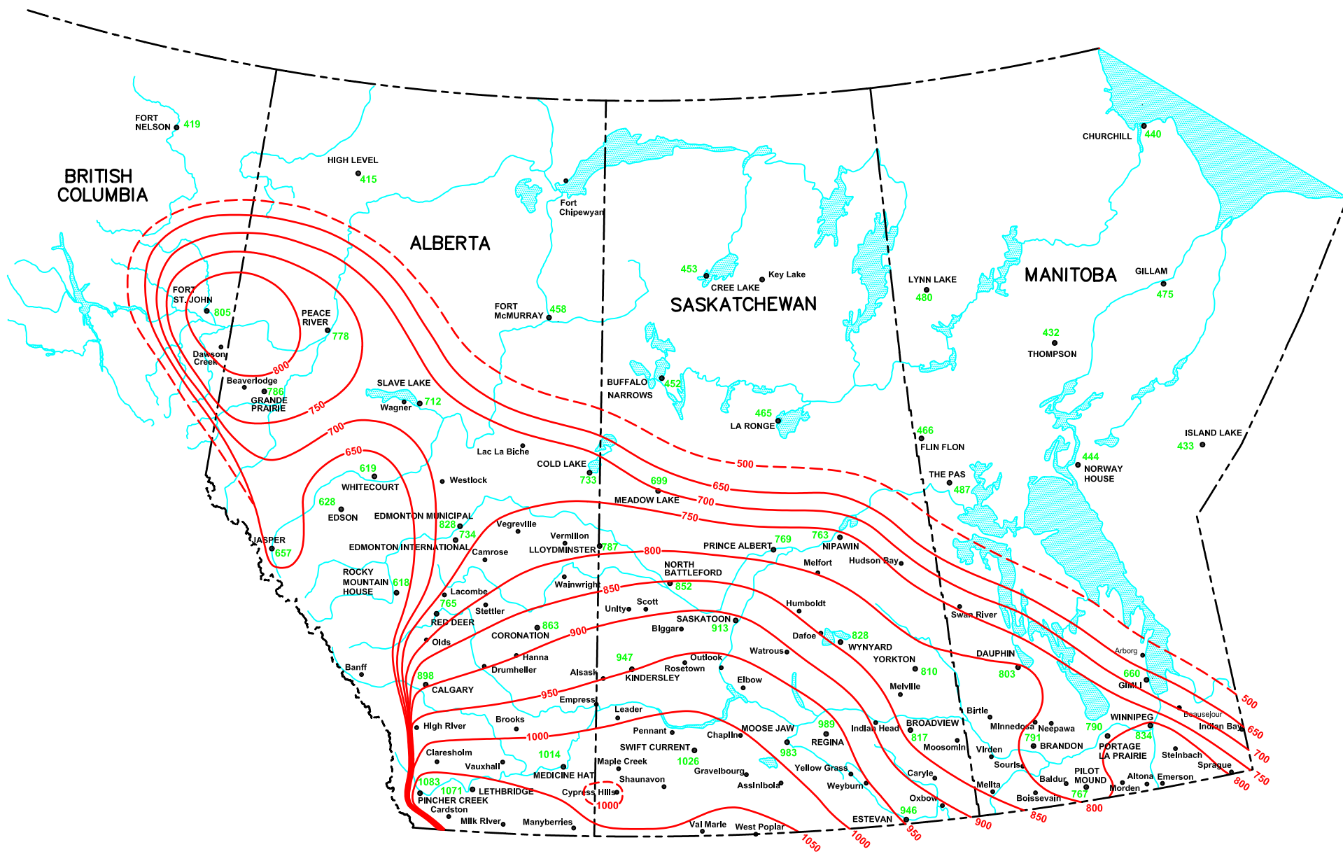
MEAN ANNUAL GROSS EVAPORATION (mm) IN THE CANADIAN PRAIRIES FOR THE STANDARD 30-YEAR PERIOD 1971-2000
